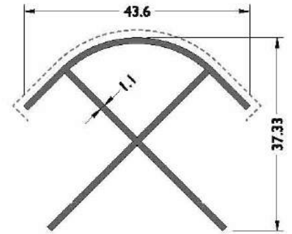
CODE / KOD THEORETICAL WEIGHT kg/m 1334 THEORETICAL WEIGHT kg/m TEORİK AĞIRLIK kg/m 0.407
